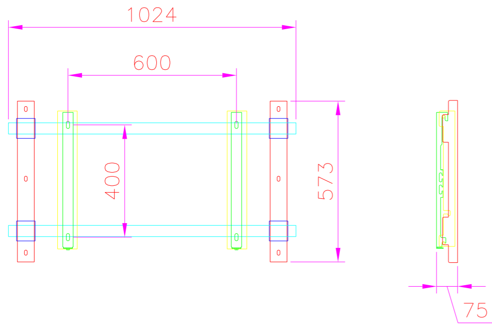
Dimension : 1023.3(W)x578(H)x75(D)mm
